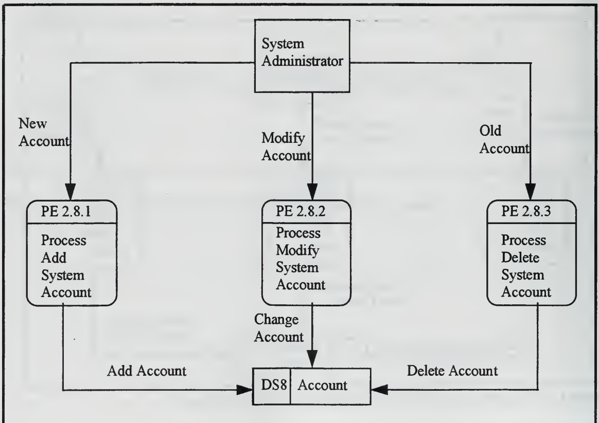
Figure 15. Primitive Level DFD For Maintaining System Account
